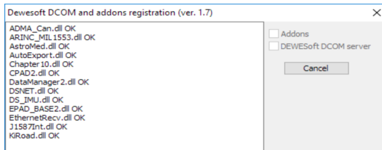
Figure 6 - addons registration
