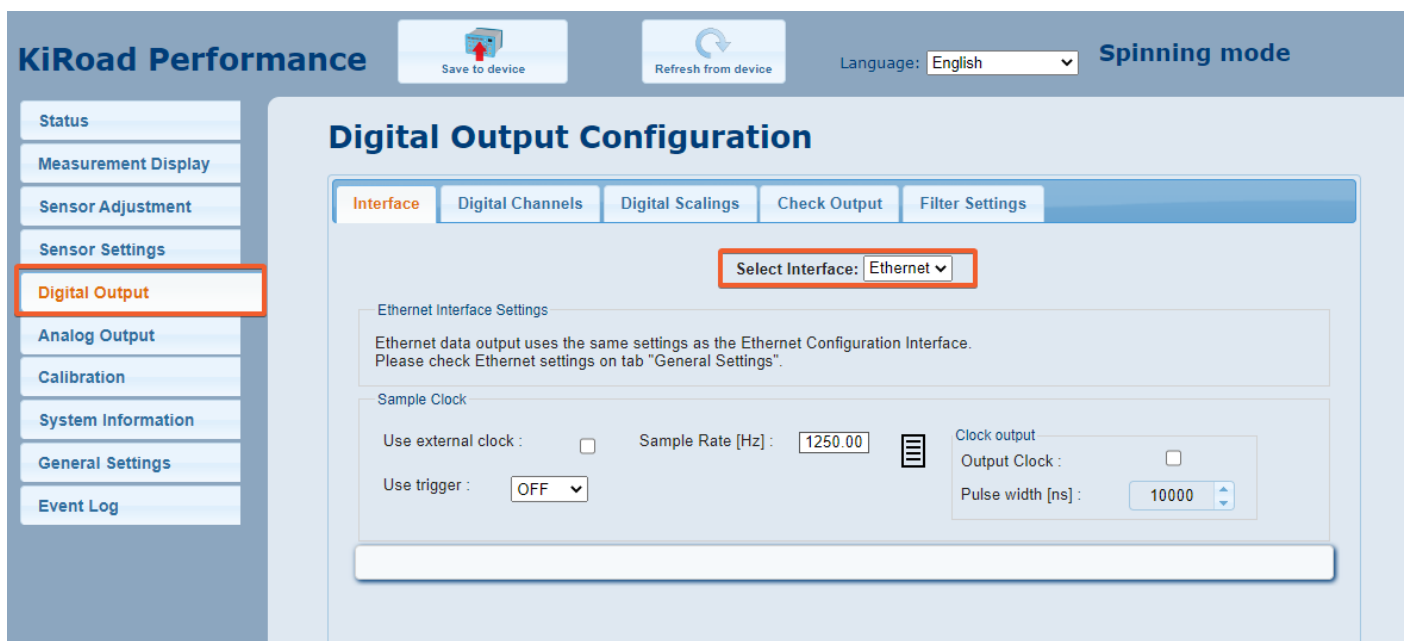
Figure 11 - Digital output setup
