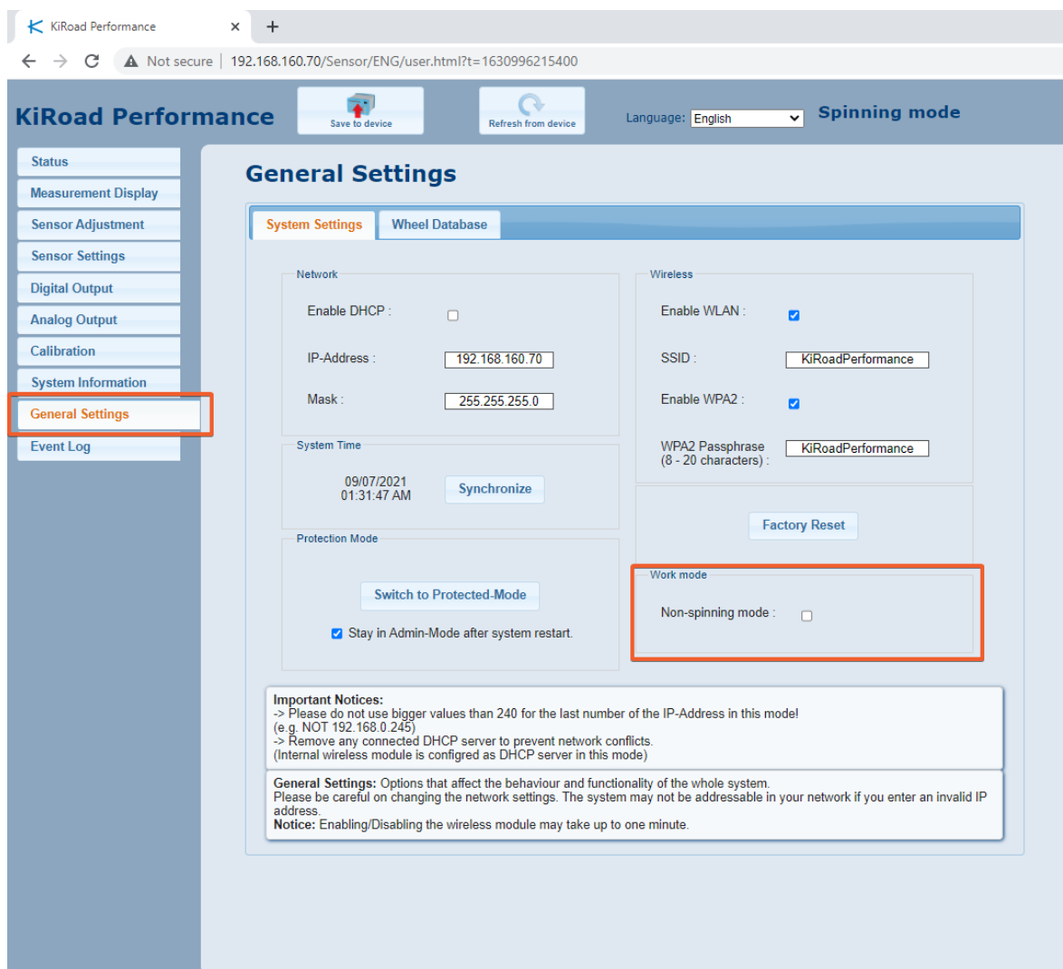
Figure 12 - General settings, Work mode box
